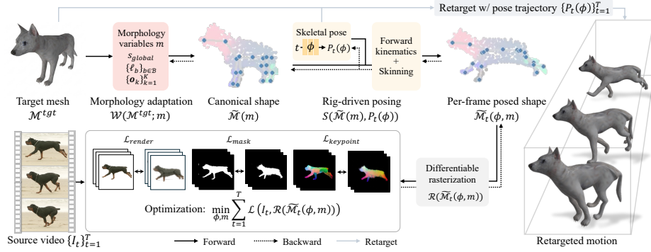
Fig. 2: Overview of MorphGS. Given a source video and a target character, MorphGS first represents the target as morphology-adaptive articulated 3D mesh (Sec. 3.2). 3D Gaussian representation is wrapped to deform pose and render differentially (Sec. 3.3). The morphology and pose parameters are jointly optimized through image-space supervision (Sec. 3.4). The recovered motion is then retargeted to the target character, yielding an animation that closely follows the source video.
